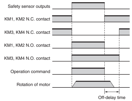
Timing chart
