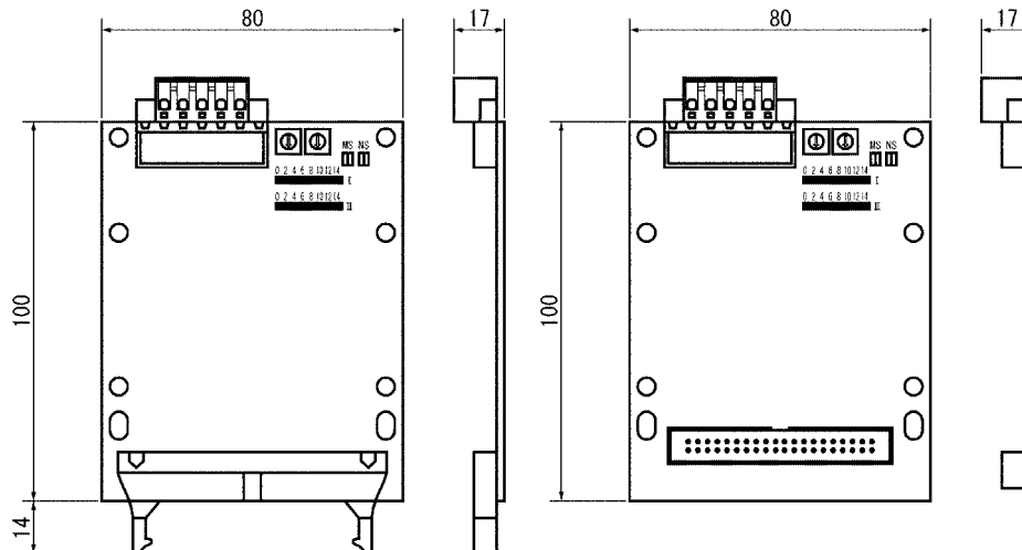
DRT2-ID32B (NPN)/DRT2-ID32B-1 (PNP) DRT2-ID32BV (NPN)/DRT2-ID32BV-1 (PNP)
