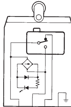
With LED Indicator (lights when operated)
