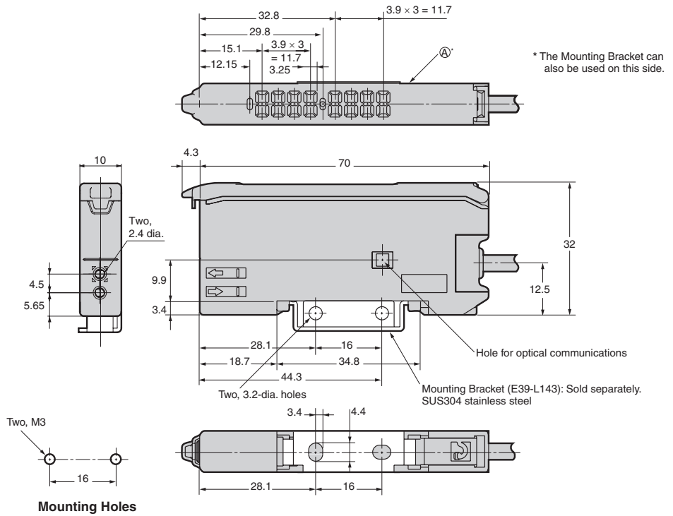
Mounting Holes
