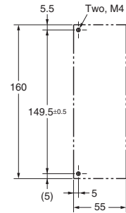
Mounting dimensions
