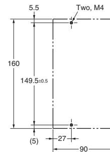
Mounting dimensions
