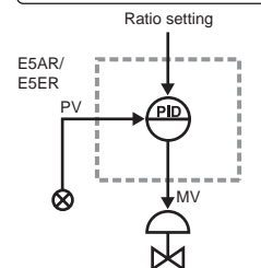
Proportional Control with a Single Unit
