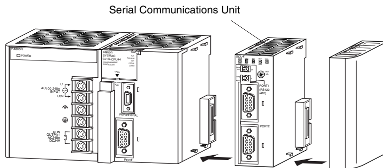
CJ1W-SCU21-V1 (Two RS-232C ports)
