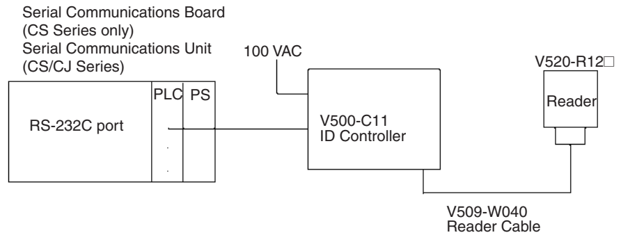
Serial Communications Unit/Board: D-sub 9 pin female
