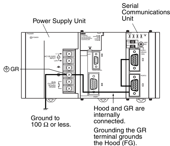
CJ-series PLC
