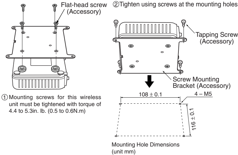
Mounting screws for this wireless unit must be tightened with torque of 4.4 to 5.3in. lb. (0.5 to 0.6N.m)
