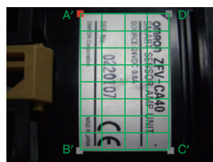
Correcting the distortion of the image based on the four points
